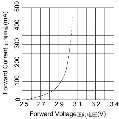
Volt-Ampere Characteristics VF-IF曲线
