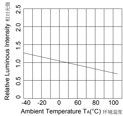
Ambient Temperature VS. Relative Intensity Ta-IV曲线
