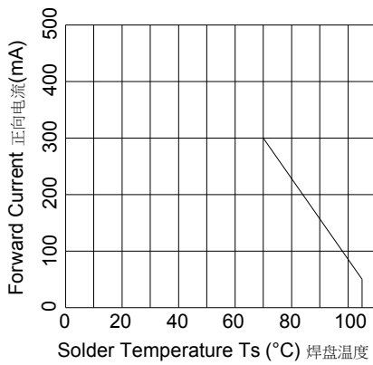
Soldering Temperature VS. Forward Current Ts-IF曲线
