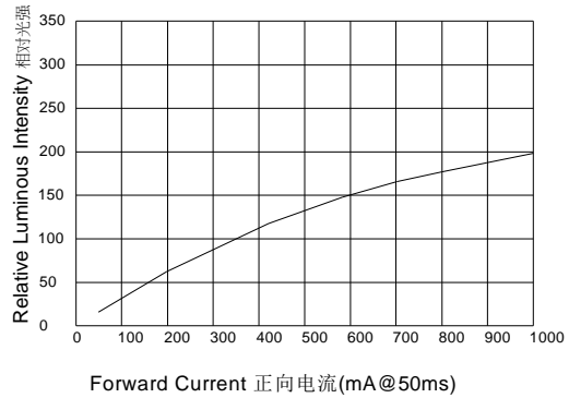
Forward Current VS. Relative Intensity IF-IV 曲线
