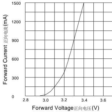
Volt-Ampere Characteristics VF-IF曲线
