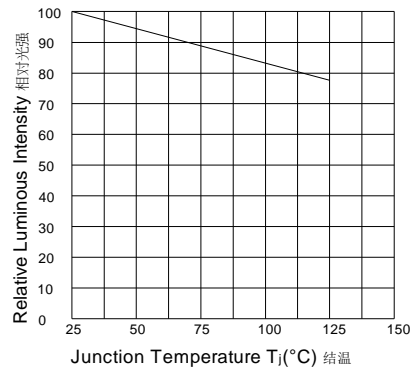
Junction Temperature VS. Relative Intensity Tj-IV 曲线
