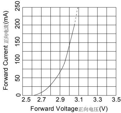
Volt-Ampere Characteristics VF-IF曲线
