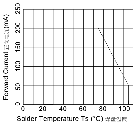
Ambient Temperature VS. Forward Current Ta-IF曲线
