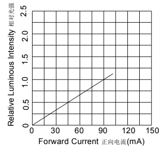
Forward Current VS. Relative Intensity IF-IV 曲线
