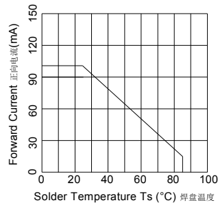
Soldering Temperature VS. Forward Current Ts-IF 曲线
