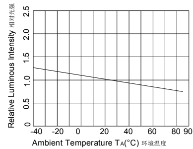
Ambient Temperature VS. Relative Intensity Ta-IV 曲线
