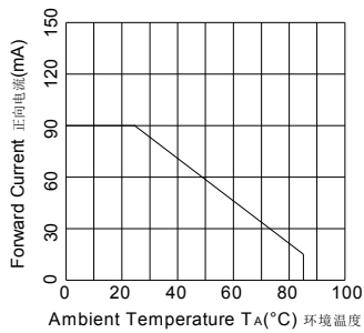
Ambient Temperature VS. Forward Current Ta-IF曲线
