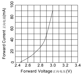
Volt-Ampere Characteristics VF-IF曲线
