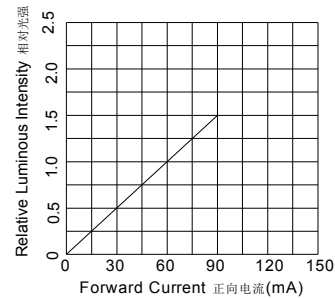
Forward Current VS. Relative Intensity IF-IV曲线
