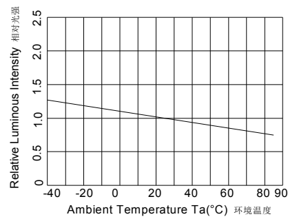
Ambient Temperature VS. Relative Intensity Ta-IV 曲线
