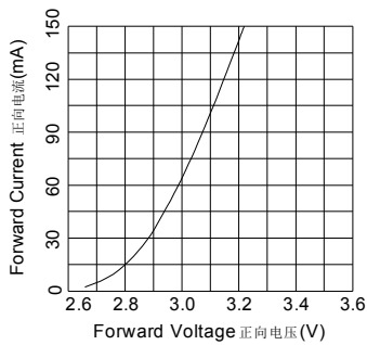
Volt-Ampere Characteristics VF-IF 曲线
