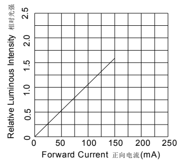
Forward Current VS. Relative Intensity IF-IV 曲线
