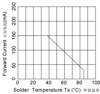
Soldering Temperature VS. Forward Current Ts-IF 曲线
