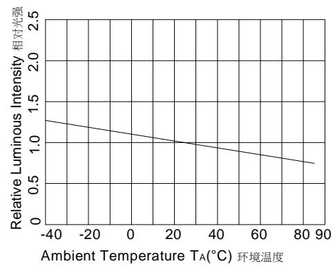
Ambient Temperature VS. Relative Intensity Ta-IV 曲线
